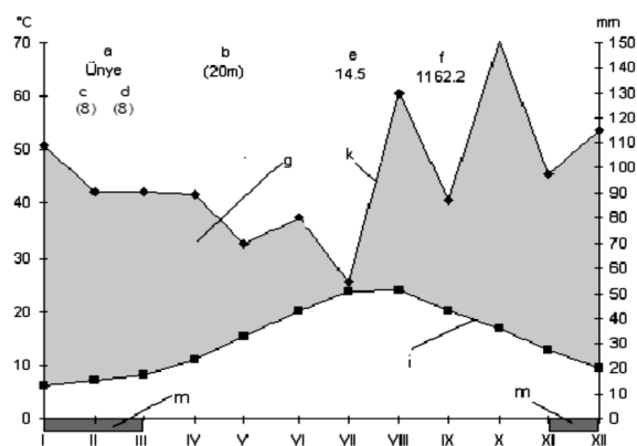
Fig. 2. Ombrothermic diagram of the study area. a. name of meteorological station, b. altitude of meteorological station (m), c. duration of temperature measurement, d. duration of rain measurement, e. annual average of temperature, f. annual average of rain, g. rainy period, i. temperature curve, k. raining curve, m. probable freezing months.
